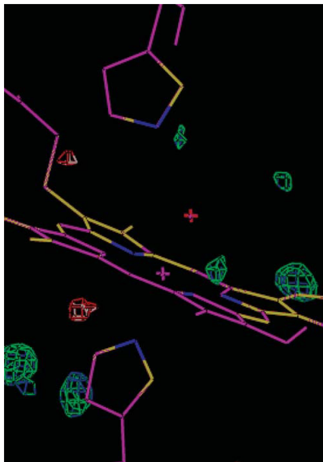
FIGURE 5 A comparison of the ComQum-X structures of the \text{Fe}^{\text{III}}\text{OH}^- HIE (magenta) and \text{Fe}^{\text{IV}}\text{OH}^- HIE models. Also included are the f_o - f_c difference maps of the two structures at the \pm 3.0\sigma level (blue and white for \text{Fe}^{\text{III}} and green and red for \text{Fe}^{\text{IV}} ).
