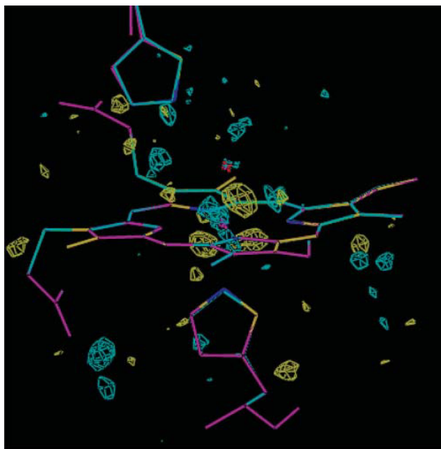
FIGURE 4 A comparison of the original crystal structure (magenta) and the re-refined structure of \text{Fe}^{\text{IV}}\text{OH}^- HIE. Also included is the f_o - f_c difference map of the original crystal structure at the \pm 3.0\sigma level (cyan and yellow).
