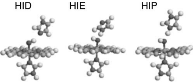
FIGURE 3 The Fe(Por)(Im)(OH - )(Im) model of the active heme site used in both the vacuum and quantum-refinement calculations. The three figures illustrate the three possible protonation states of the distal His model—HID, HIE, and HIP.
